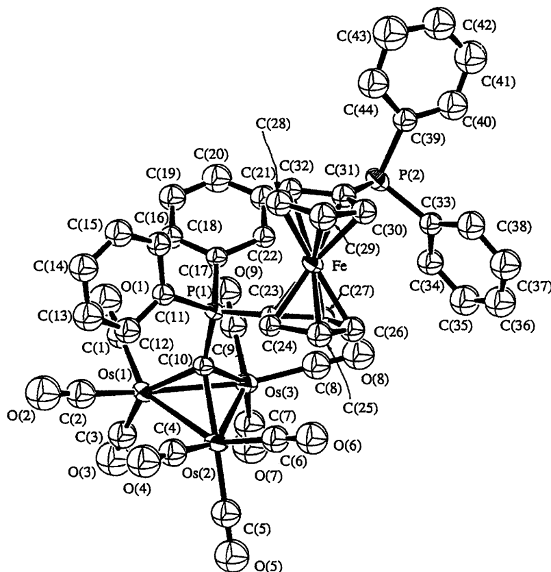
Fig. 5 The molecular structure of [\text{Os}_3(\mu\text{-H})_2(\text{CO})_9\{\mu_3\text{-CPh}_2(\eta^5\text{-C}_5\text{H}_4)\text{Fe}(\eta^5\text{-C}_5\text{H}_4\text{PPh}_2)\}]_3
