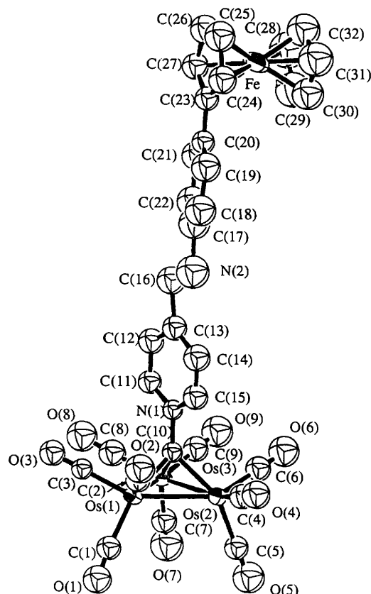
Fig. 4 The molecular structure of [\text{Os}_3(\mu\text{-H})_2(\text{CO})_9\{\mu_3\text{-CNC}_5\text{H}_4\text{CH}=\text{NC}_6\text{H}_4(\eta^5\text{-C}_5\text{H}_4)\text{Fe}(\eta^5\text{-C}_5\text{H}_5)\}] 2
